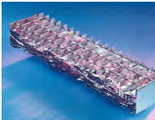
Darflare™ cross-section showing the load-bearing grating and underlying contoured foils.
